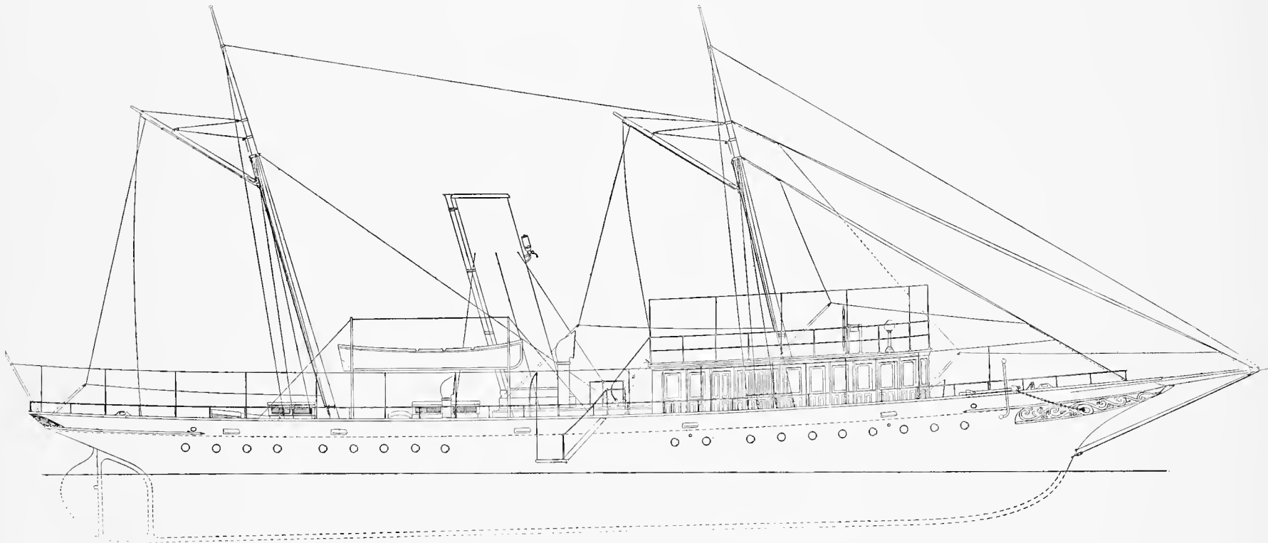
MRS. LUCY C. CARNEGIE'S STEAM YACHT DUNGENESS.—Built by the Maryland Steel Co., Sparrow's Point, Md.
